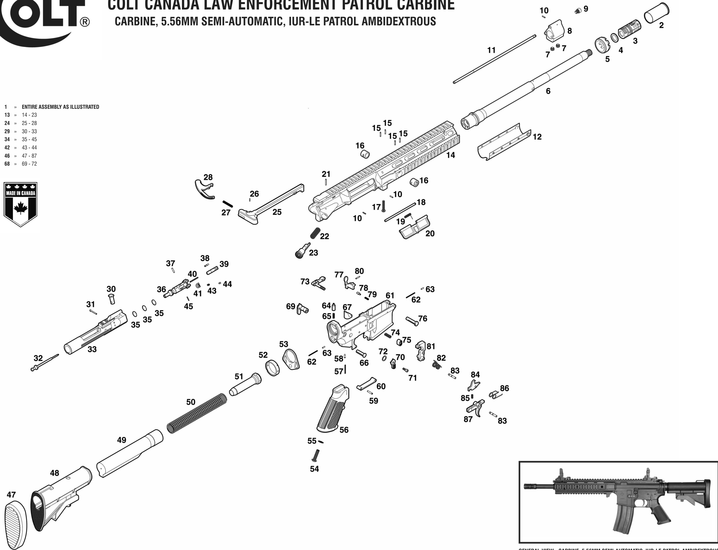
GENERAL VIEW - CARBINE, 5.56MM SEMI-AUTOMATIC, IUR-LE PATROL AMBIDEXTRIOUS
